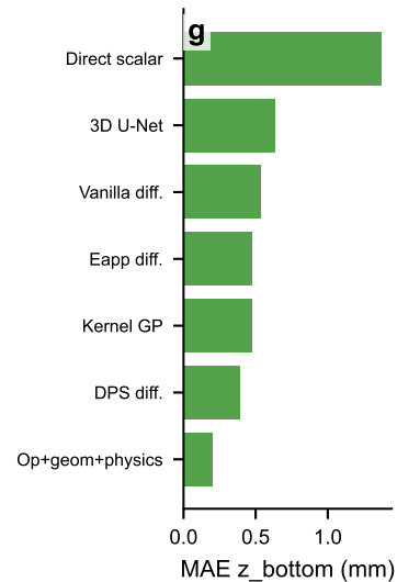
Held-out depth benchmark
